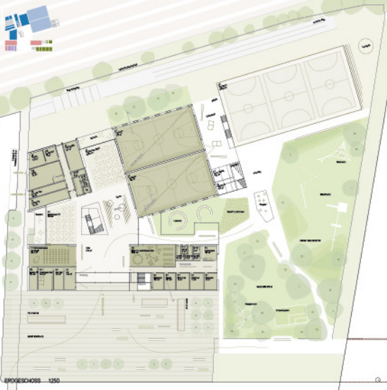
ERDGESCHUSS 1250
